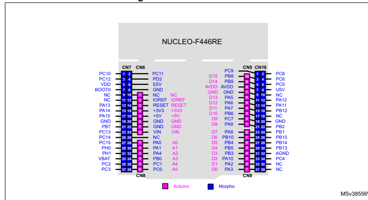
Figure 25. NUCLEO-F446RE
