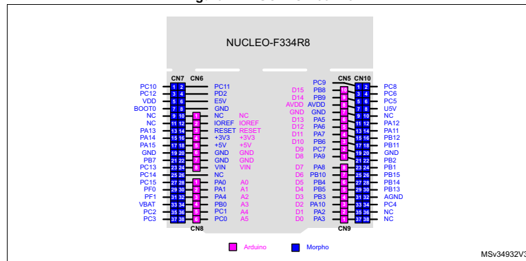
Figure 17. NUCLEO-F334R8
