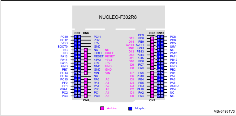
Figure 15. NUCLEO-F302R8
