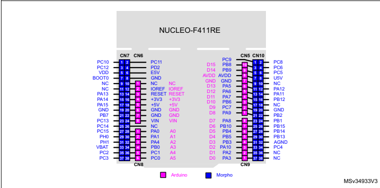
Figure 19. NUCLEO-F411RE
