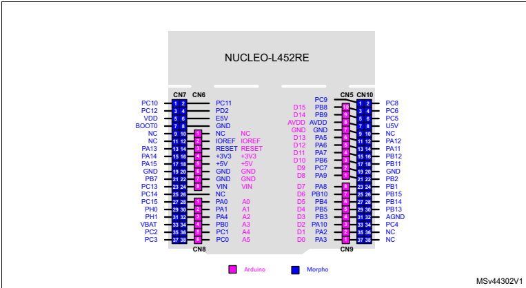
Figure 23. NUCLEO-L452RE
