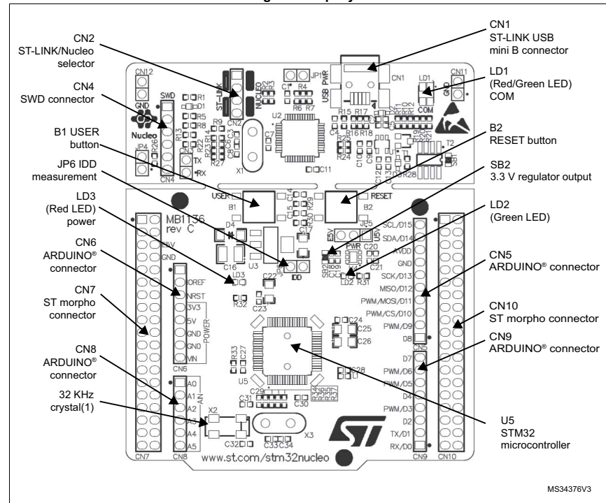
Figure 3. Top layout
