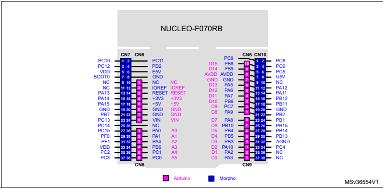
Figure 11. NUCLEO-F070RB
