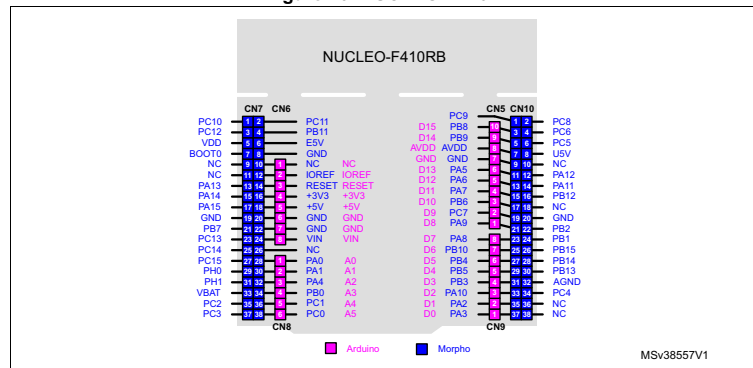
Figure 26. NUCLEO-F410RB
