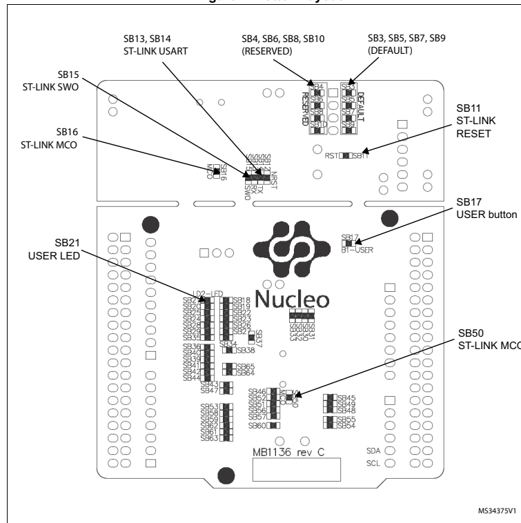
Figure 4. Bottom layout
